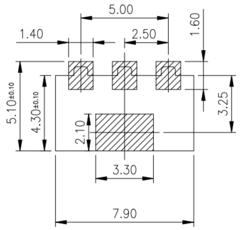
RECOMMENDED PCB LAYOUT TOP VIEW (.XX±0.05)
